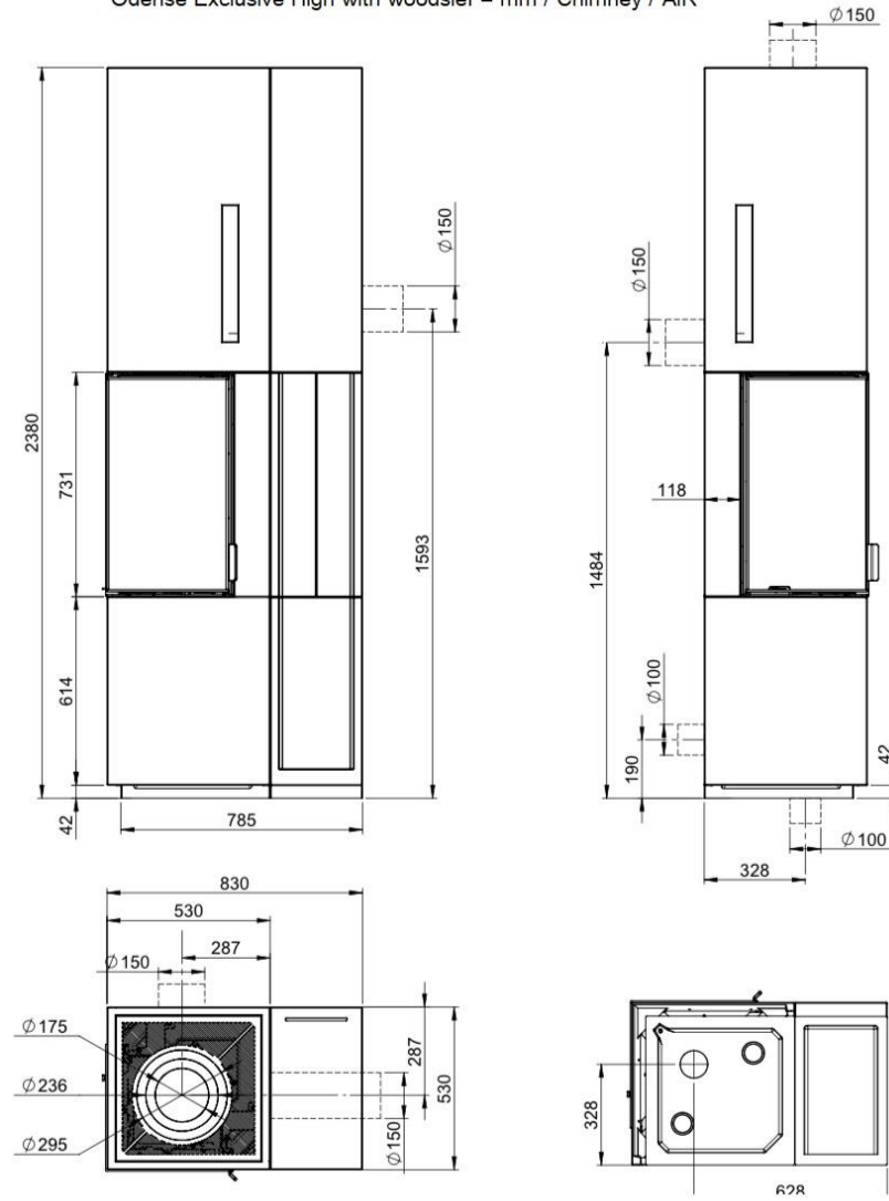
Odense Exclusive High with woodslef = mm / Chimney / AIR
